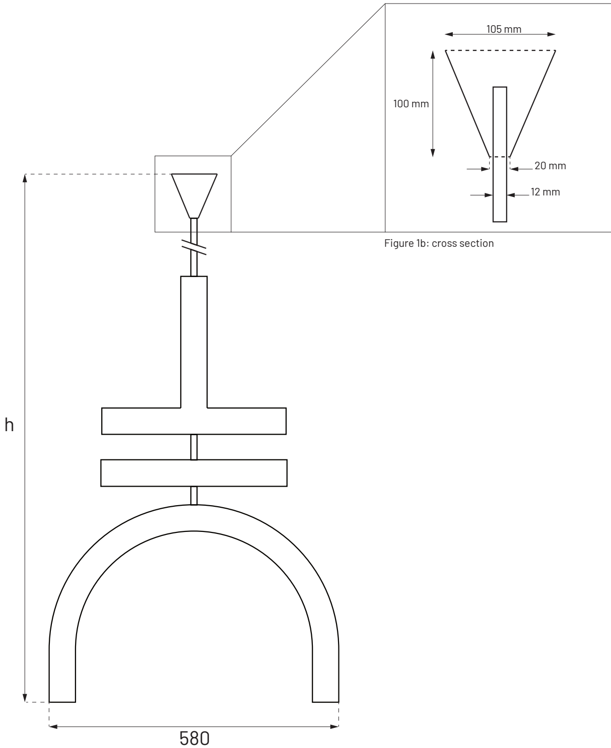
Figure 1: TRN dimensions
